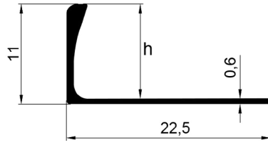
ALÜMİNYUM EKO FAYANS BİTİM PROFİLİ Aluminum Eco Tile Finishing Profile
