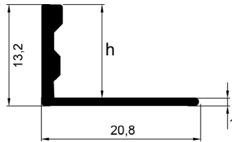
ALÜMİNYUM ULTRA LÜKS FAYANS BİTİM PROFİLİ Aluminum Ultra Luxury Tile Finishing Profile
