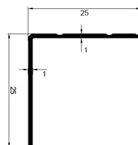
ALÜMİNYUM L MERDİVEN BASAMAK PROFİLİ Aluminum L Stair Step Profile
