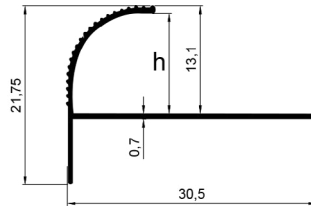
ALÜMİNYUM Ç MERDİVEN BASAMAK PROFİLİ Aluminum Fence Stair Step Profile
