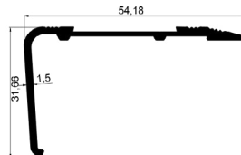
ALÜMİNYUM LÜKS LASTİKLİ MERDİVEN BASAMAK PROFİLİ Aluminum Luxury Rubber Ladder Step Profile
