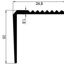
ALÜMİNYUM L MERDİVEN BASAMAK PROFİLİ Aluminum L Stair Step Profile
