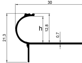
ALÜMİNYUM Ç MERDİVEN BASAMAK PROFİLİ Aluminum Fence Stair Step Profile
