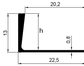
ALÜMİNYUM LÜKS FAYANS BİTİM PROFİLİ Aluminum Luxury Tile Finishing Profile
