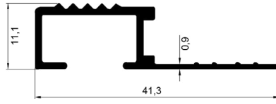
ALÜMİNYUM KLASİK MERDİVEN BASAMAK PROFİLİ Aluminum Classic Stair Step Profile
