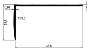
ALÜMİNYUM L MERDİVEN BASAMAK PROFİLİ Aluminum L Stair Step Profile
