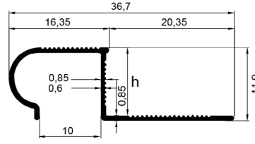
ALÜMİNYUM OVAL MERDİVEN BASAMAK PROFİLİ Aluminum Oval Stair Step Profile
