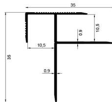
ALÜMİNYUM F MERDİVEN BASAMAK PROFİLİ Aluminum F Stair Step Profile
