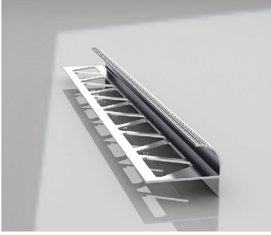
ALÜMİNYUM F MERDİVEN BASAMAK PROFİLİ Aluminum F Stair Step Profile
