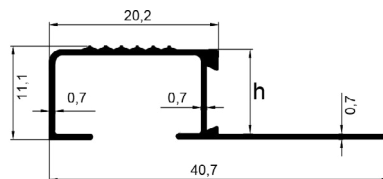
ALÜMİNYUM KLASİK MERDİVEN BASAMAK PROFİLİ Aluminum Classic Stair Step Profile
