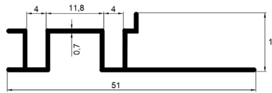
ALÜMİNYUM LASTİKLİ MERDİVEN BASAMAK PROFİLİ Aluminum Rubber Ladder Step Profile
