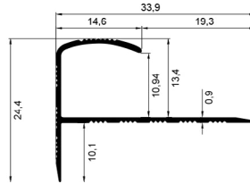
ALÜMİNYUM F MERDİVEN BASAMAK PROFİLİ Aluminum F Stair Step Profile
